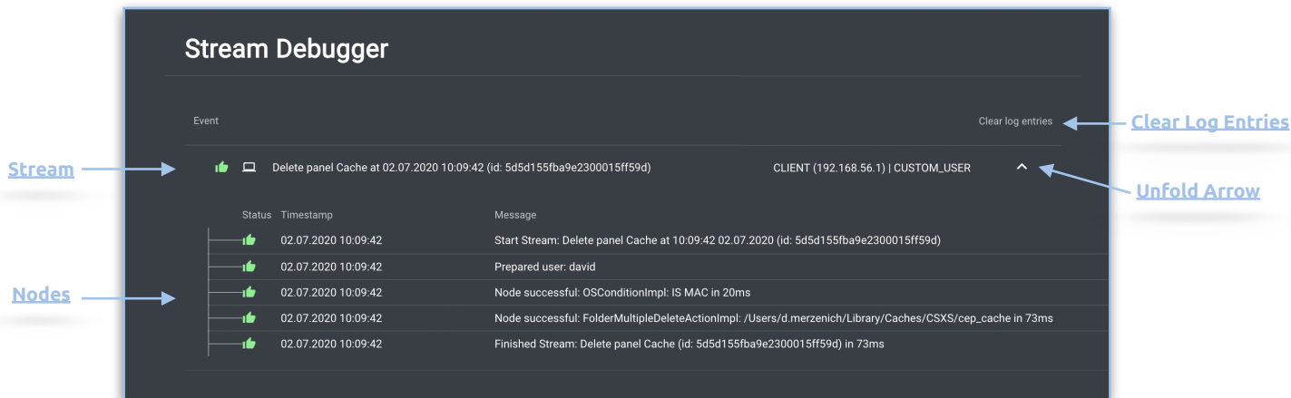
Figure 2.11.3. Stream debugger
