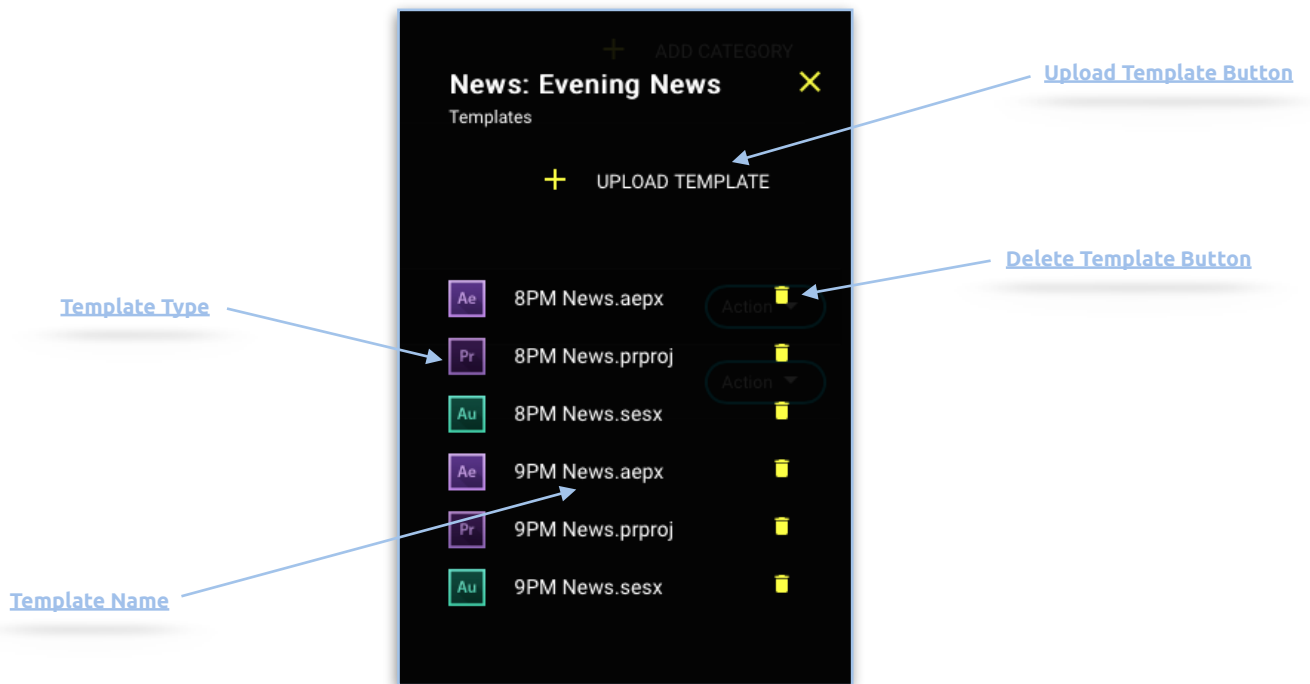
Figure 2.7.3 hidden overlay
