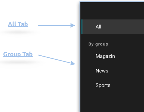
Figure 2.7.1 sidebar menu
