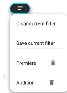
Figure 1.3.6 Personal Filter
