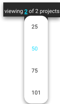
Figure 1.3.9 Pagination
