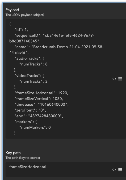
Figure 3.2.2 JSON Extract
