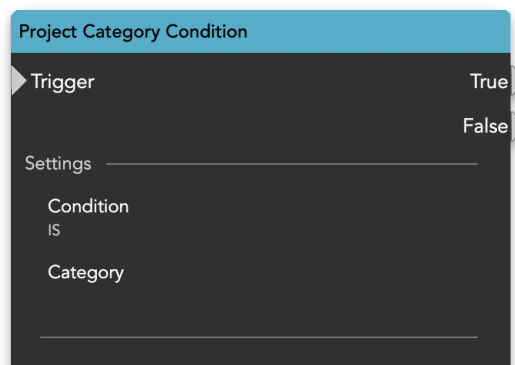
Figure 2.1. Condition Node
