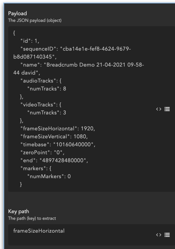
Figure 3.2.2 JSON Extract
